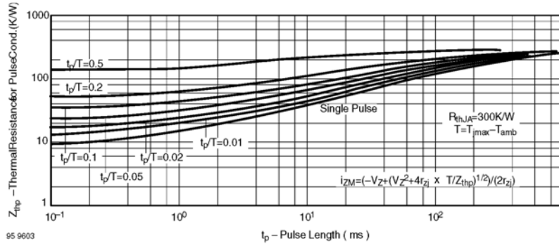
Fig. 13 Thermal Response
